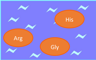
primordial soup
